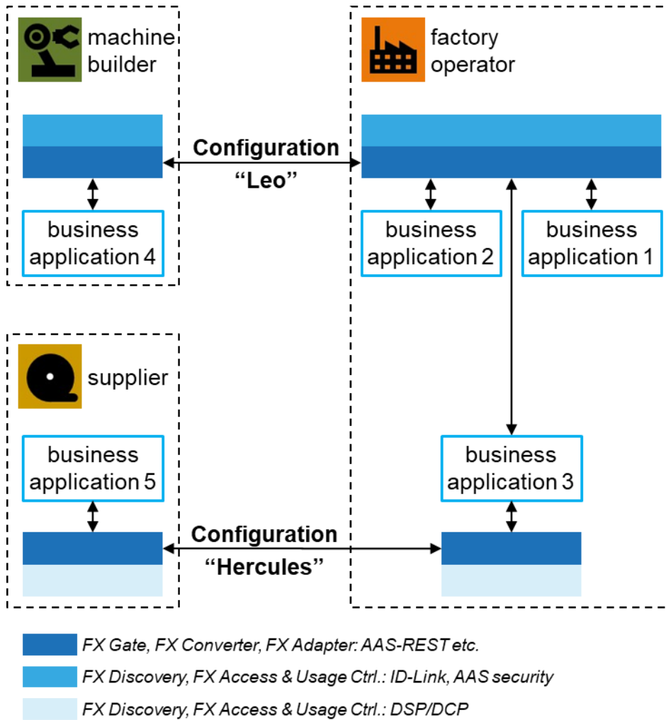
Figure 7: Combining different configurations of the MX-Port (Source: Factory-X)
